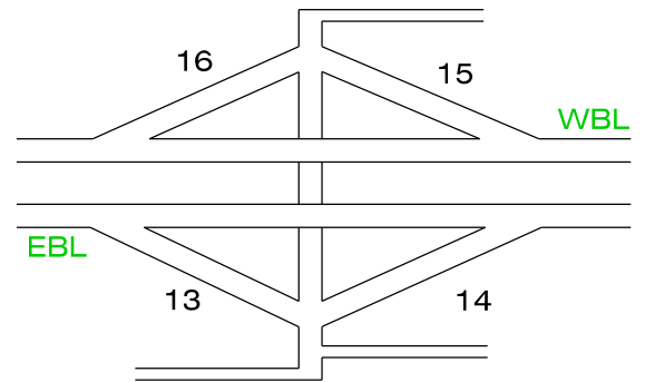
Divide Interchange
