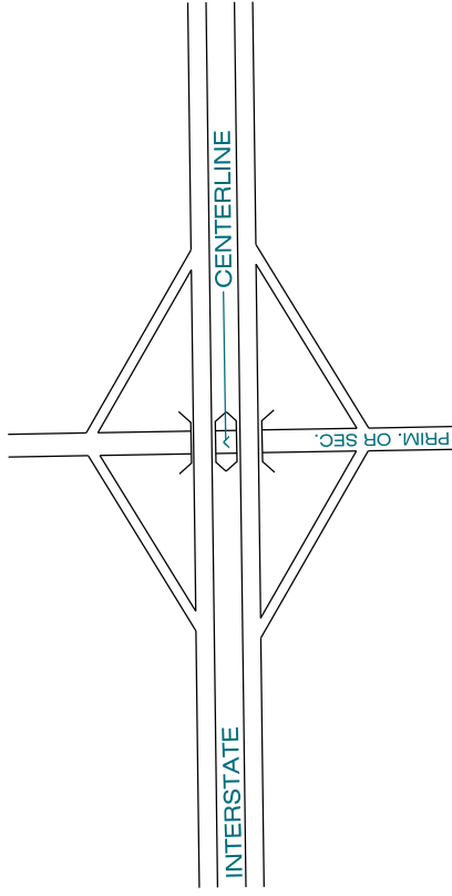
SEPARATED INTERSECTIONS
